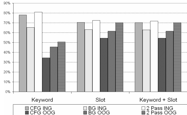
Figure 2. The semantic accuracies comparing the baseline CFG against both the BG (backoff grammar alone) and the two-pass approach (CFG + Backoff) separated into functional constituent groups and further separated by ING and OOG commands.
