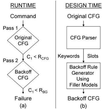
Figure 1. (a) A two-pass approach which leverages a base CFG for ING recognition and a backoff grammar for failed utterances. (b) Design time procedure for generating a backoff grammar
